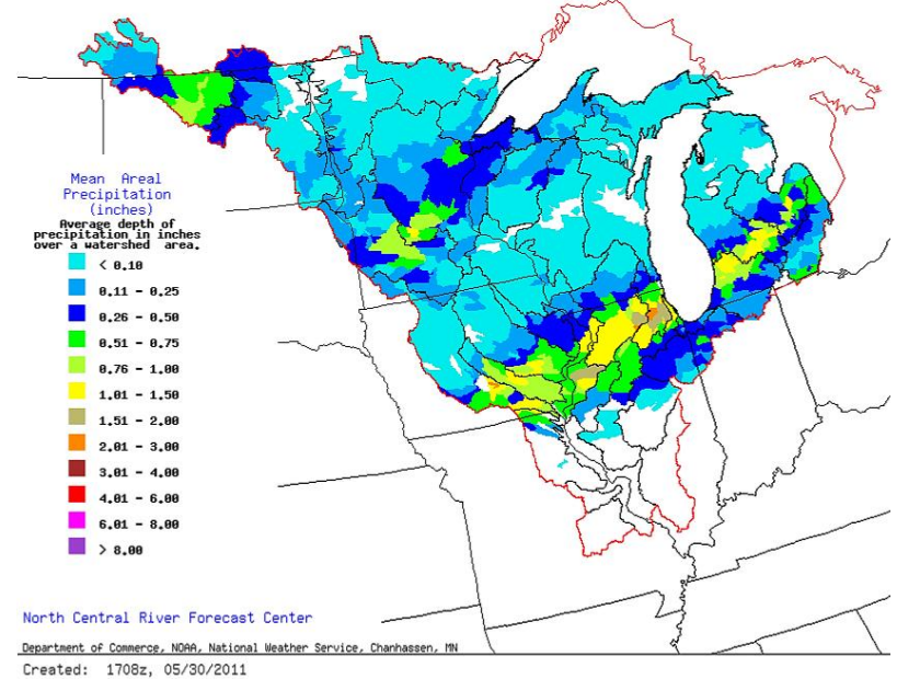
Mean Areal Precipitation 24 hour total ending 12Z, May 30, 2011
